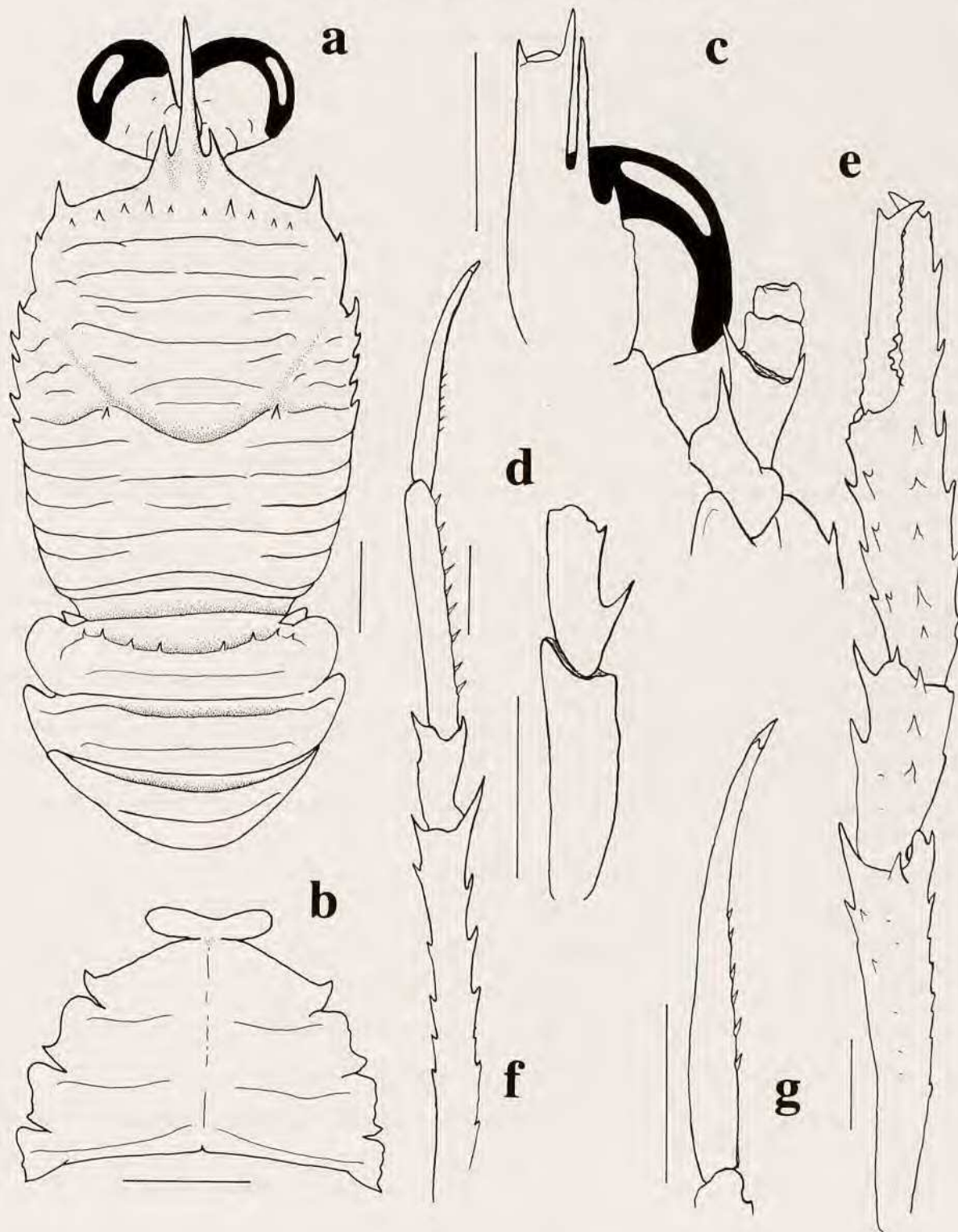
FIG. 1. — Munida parca sp. nov., ov. ♀ 4.3 mm, holotype from Stn 705 (BATHUS 1): a, carapace, dorsal view; b, sternal plastron; c, ventral view of cephalic region, showing antennula and antennal peduncles; d, right third maxilliped, lateral view; e, left cheliped, dorsal view; f, right first walking leg, lateral view; g, dactylus of right first walking leg, lateral view. Scales = 1 mm.
